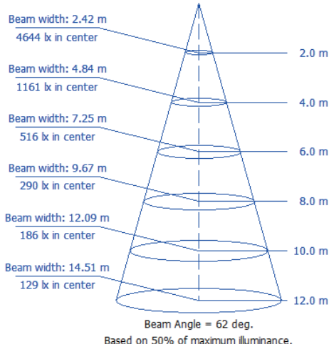
CJF-200S
